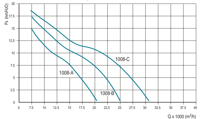
DUCT-M 1000 - 8 poles
