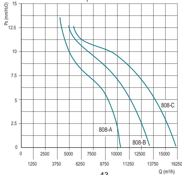
DUCT-M 800 - 8 poles
