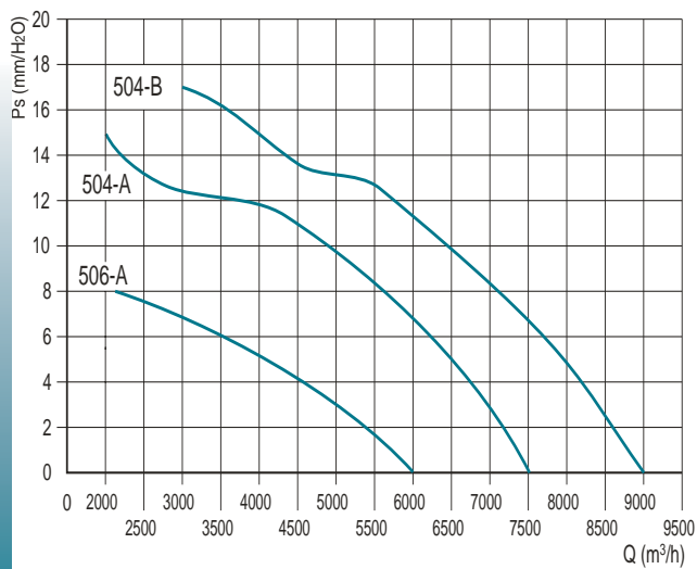
DUCT-M 500
