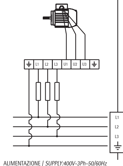
SCHEMA COLLEGAMENTO WIRING DIAGRAM
